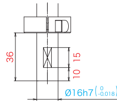
■ Detailed drawing of End-effector mounting face
