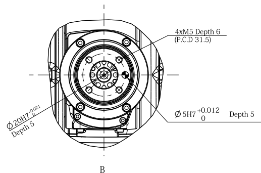
Detailed drawing of end-effector mounting face
